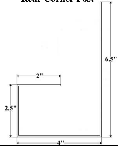
Part GR3-1 (108'')- Grumman Rear Corner Post
